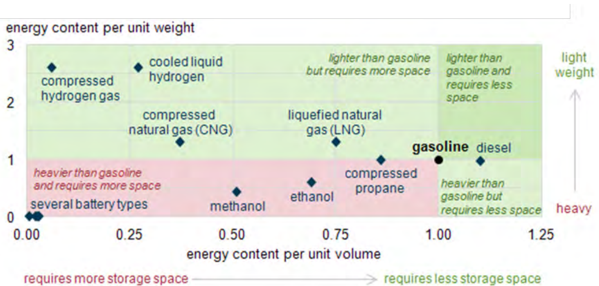
Figure 1: Energy density comparison of selected fuels (indexed to gasoline = 1) (21)
