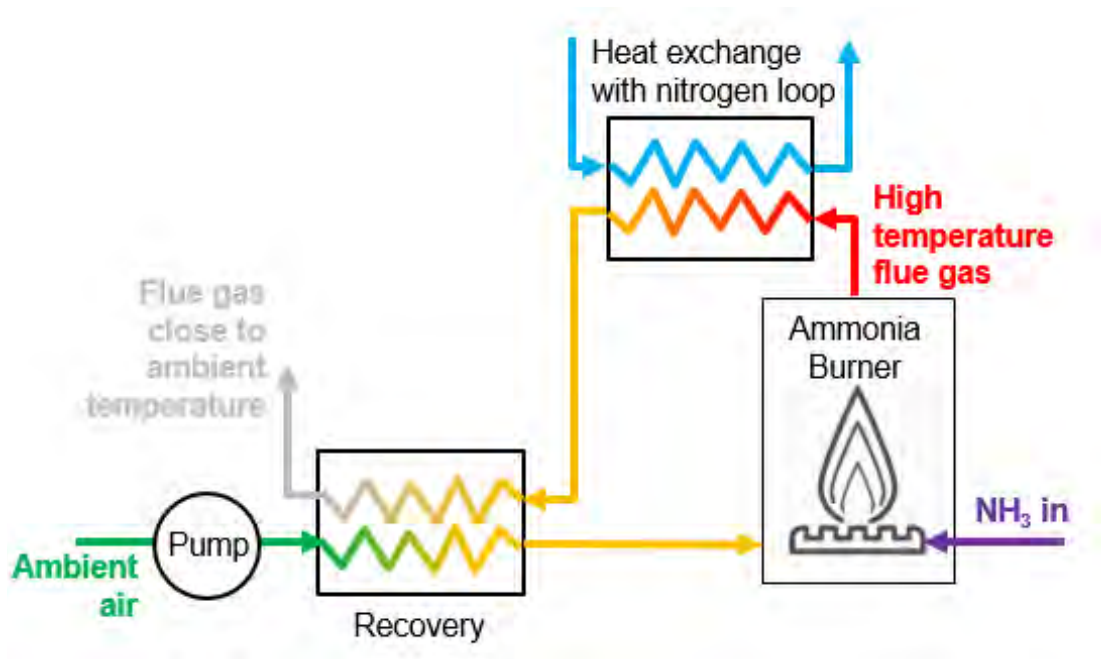
Figure 24: Schematic of ammonia burner for efficient large scale cracking
